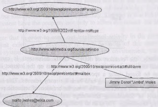
Fig. 6.7 – Wikipedia founder business card graph
