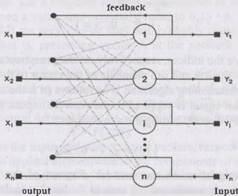
Fig. 4.11 – Block diagram of the Hopfield network
