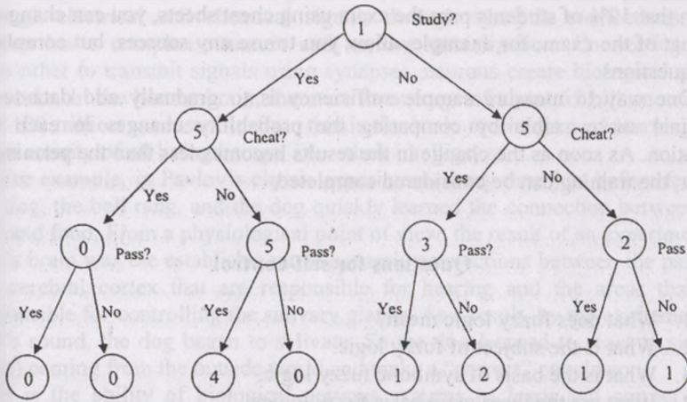
Fig. 3.1 – Observation tree
