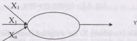
Fig. 4.1 – Single neuron
