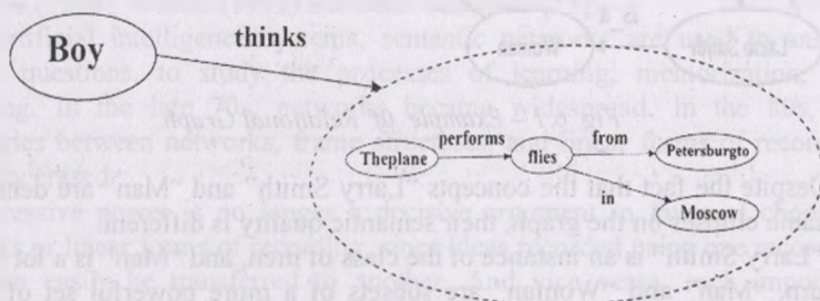
Fig. 6.3 – Conceptual graph
