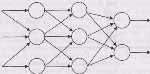
Fig. 4.2 – Neural network
