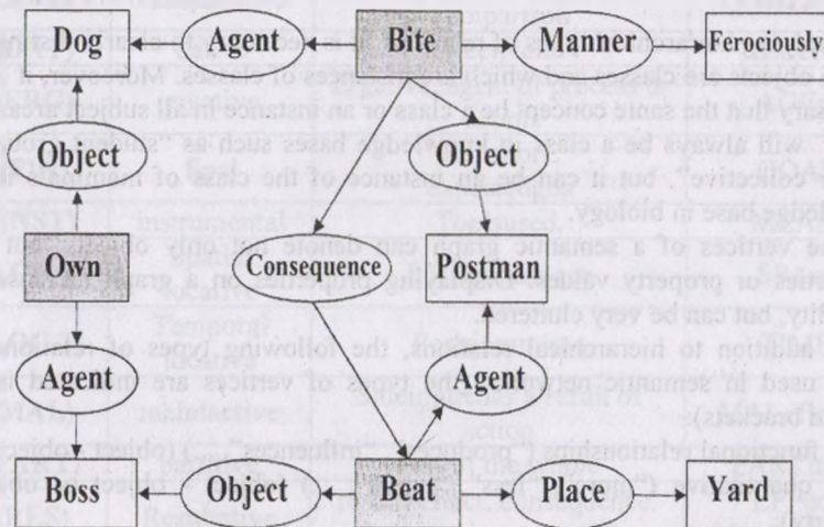
Fig. 6.5 – Semantic Network "Postman"
