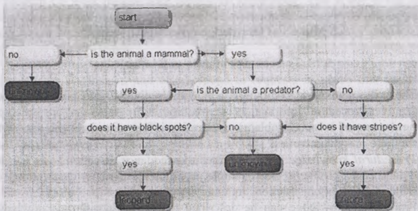
Fig. 5.1 – Example of rules submission
