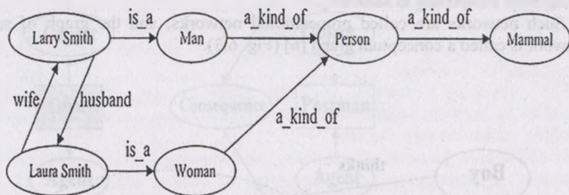
Fig. 6.1 – Example of Relational Graph
