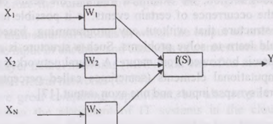
Fig. 4.3 – Neuron structure
