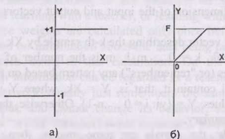
Fig. 4.12 – Activation functions
